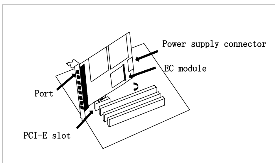
Figure 4 Hardware setup
