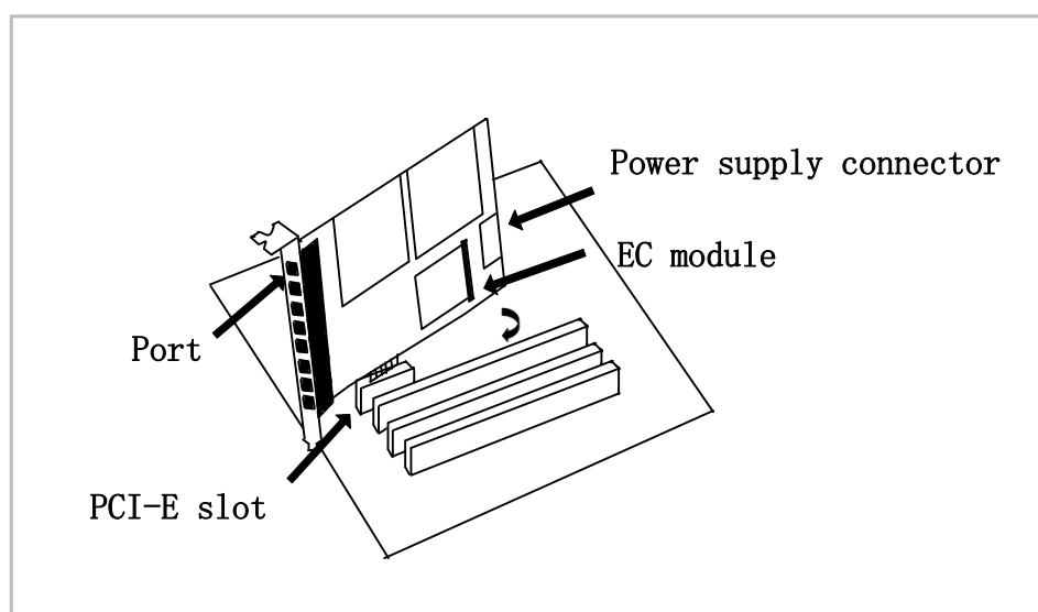
Figure 4 Hardware setup
