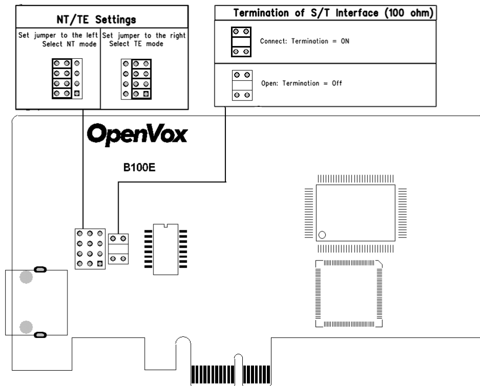
Figure 3 Jumper setting
