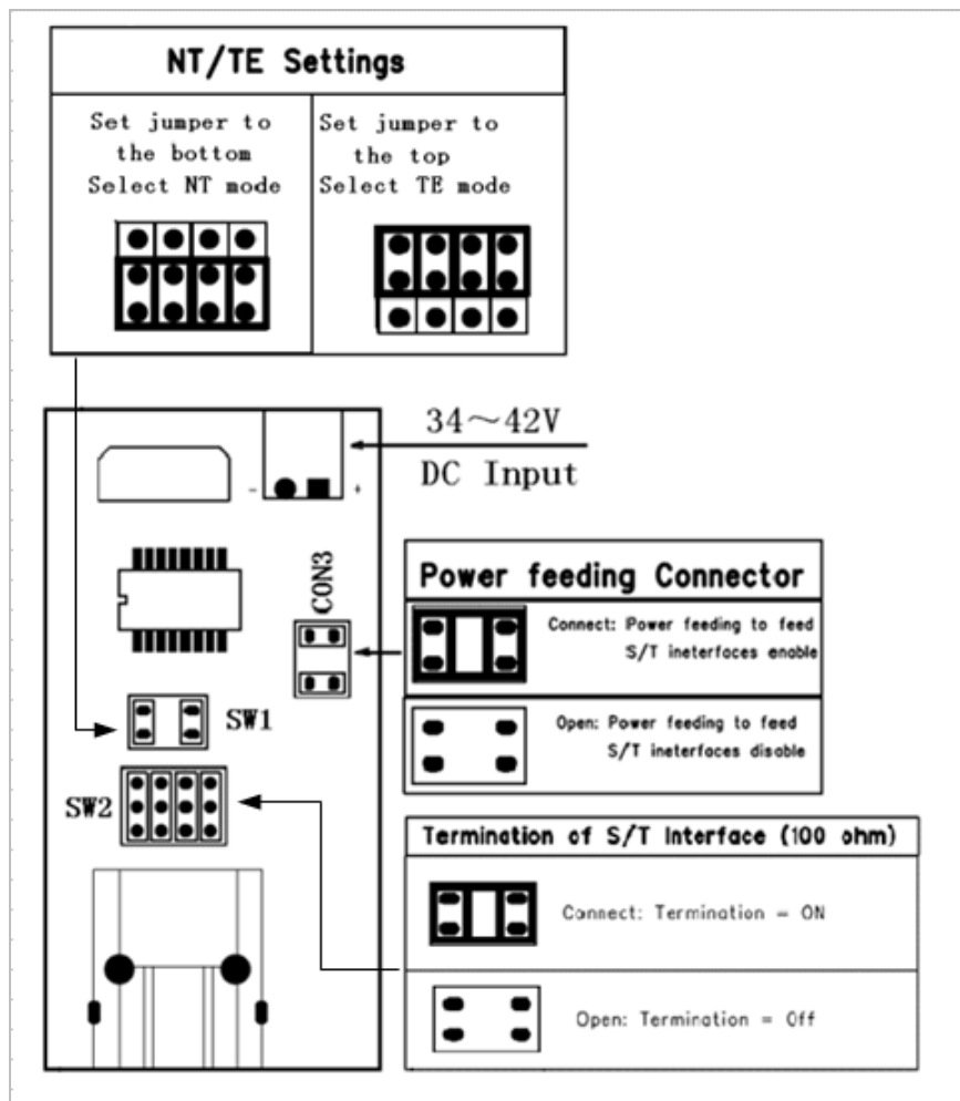
Figure 3 Jumper settings
