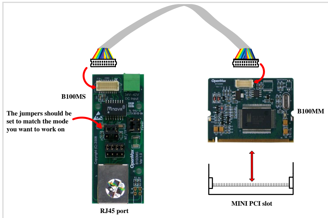
Figure 4 Cable connector
