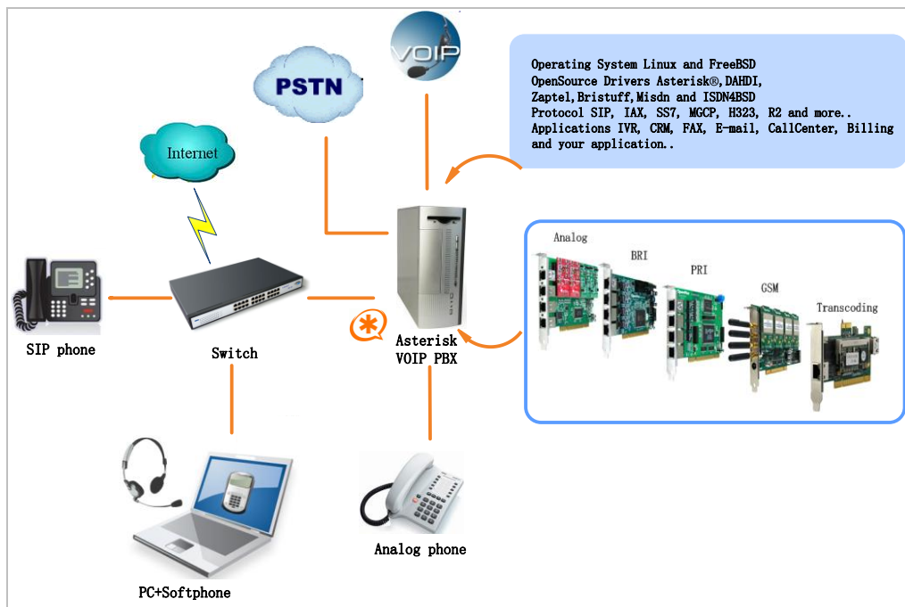
Figure 1 Topology
