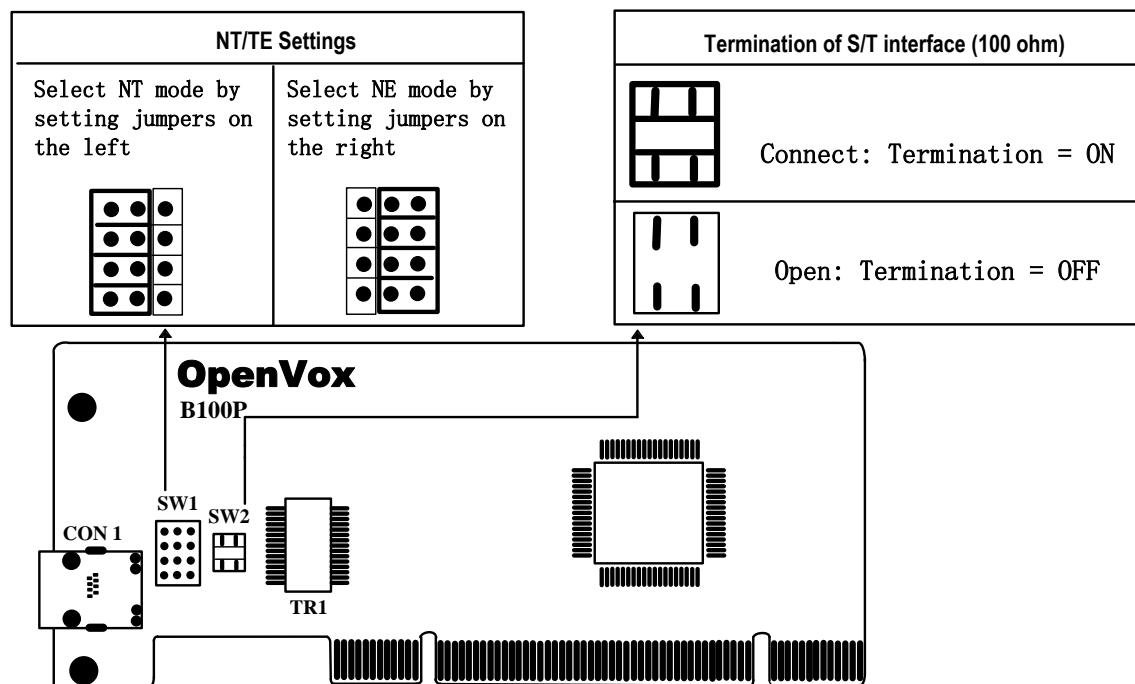
Figure 3 Jumper setting
