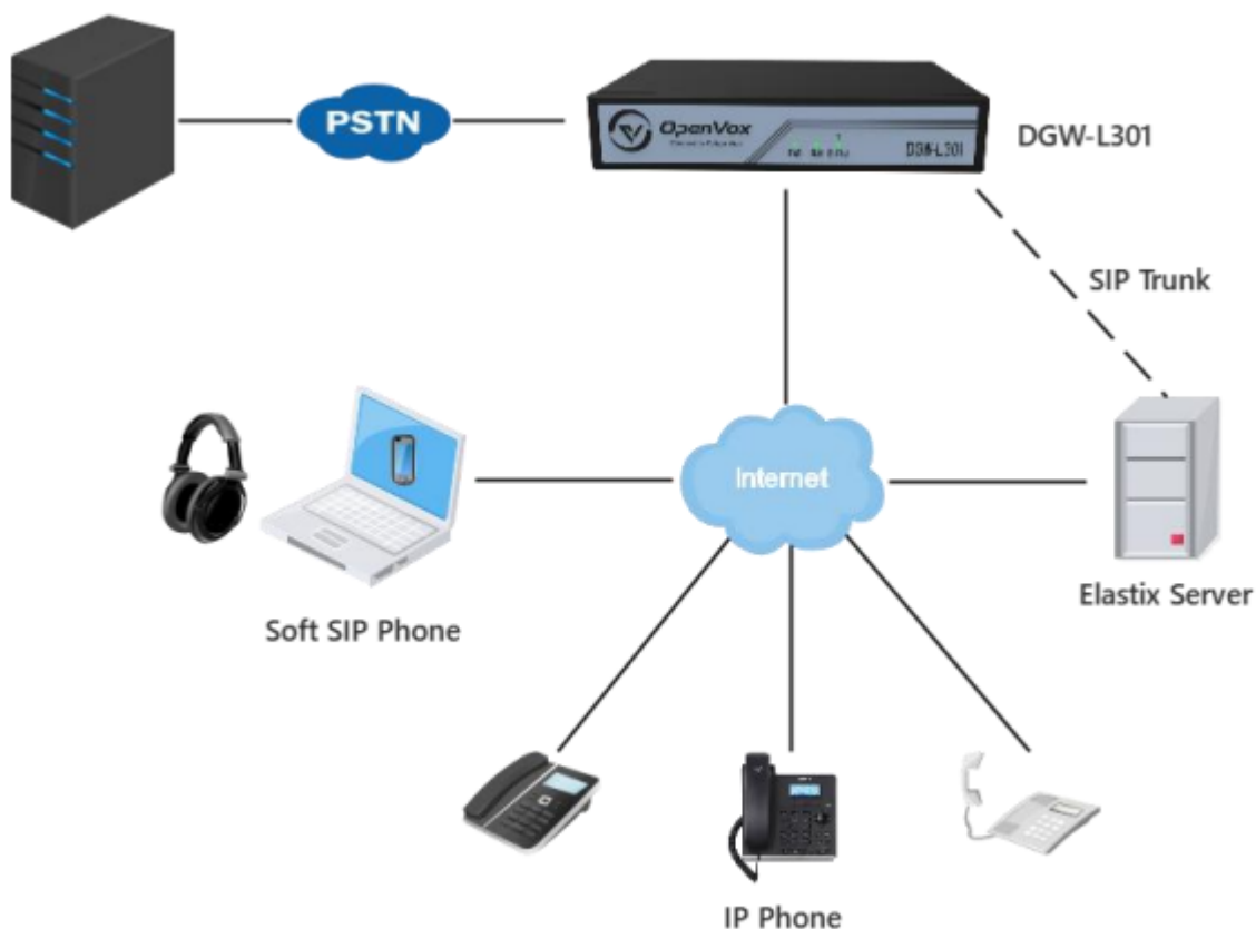
Figure 1-2-1 Application Topology
